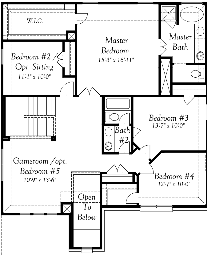
SECOND FLOORPLAN
