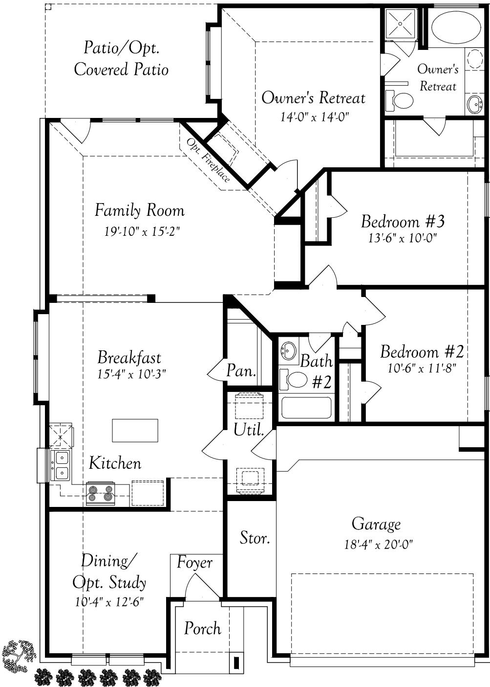
FLOORPLAN
