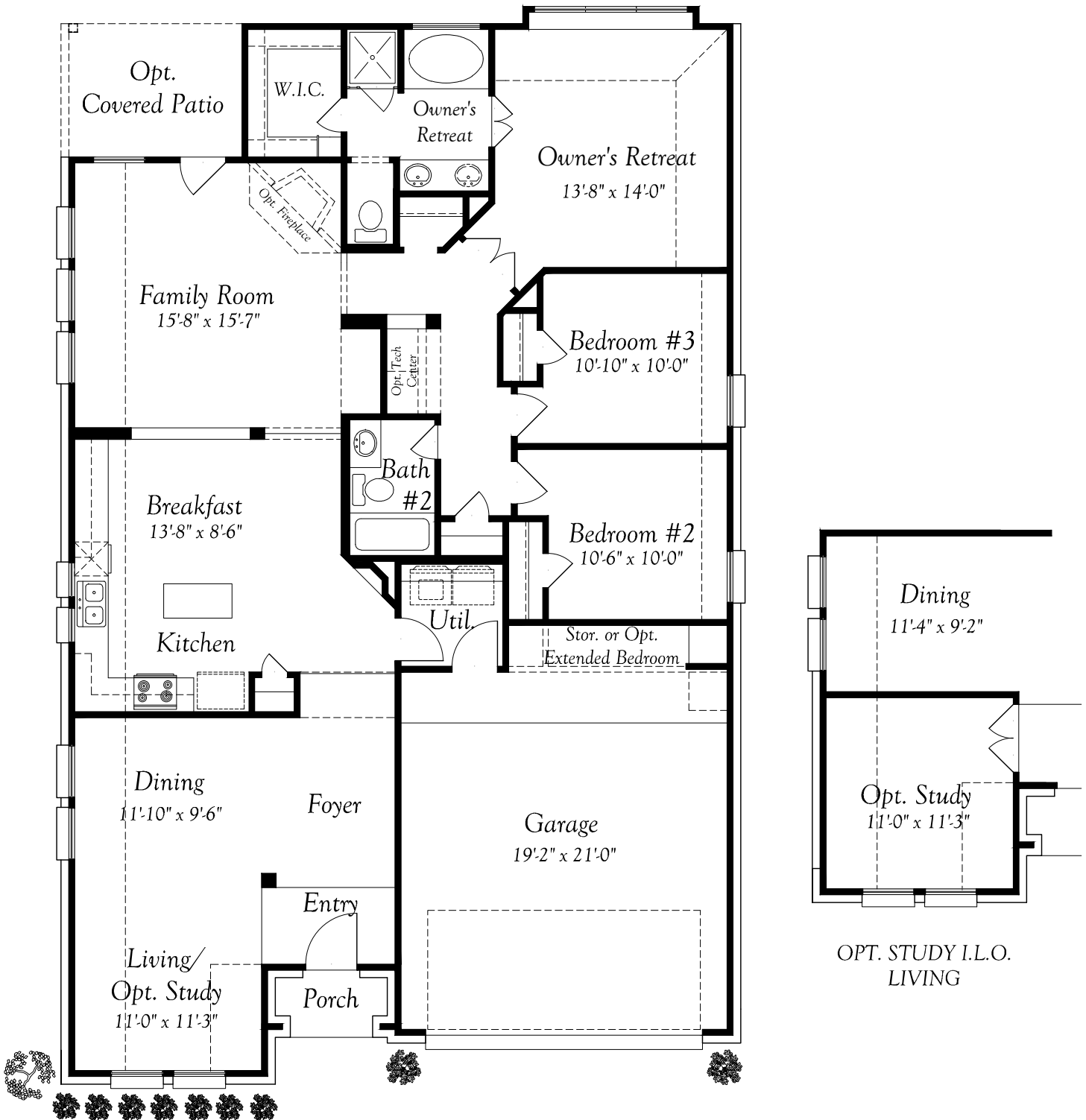
FLOORPLAN
